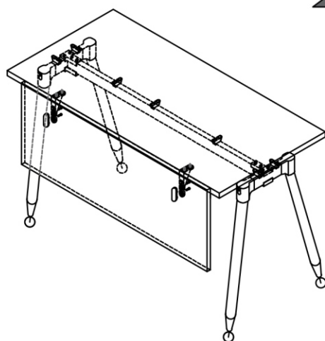
DRILLING DIAGRAM WITH TABLE TOP
